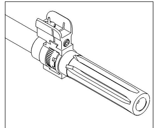
Adjustable Front Sight Tower for M14 / M1A
